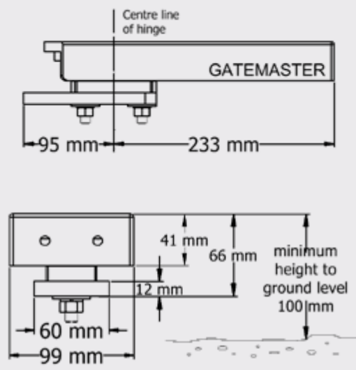
APSTOP SHOWN IN GATE
